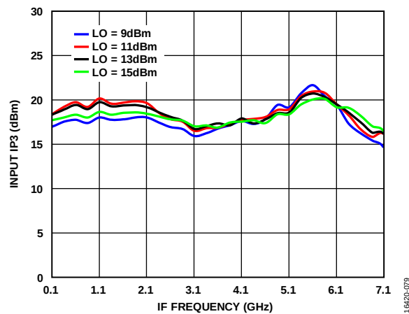
Figure 77. Input IP3 vs. IF Frequency at Various LO Power Levels, T_A = 25^\circ\text{C}
