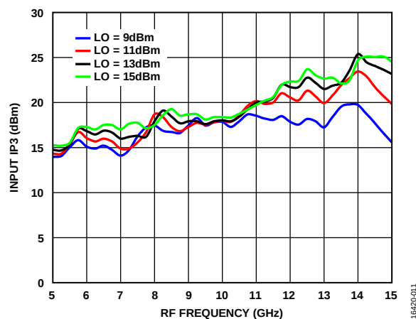
Figure 10. Input IP3 vs. RF Frequency at Various LO Power Levels, T_A = 25^\circ\text{C}
