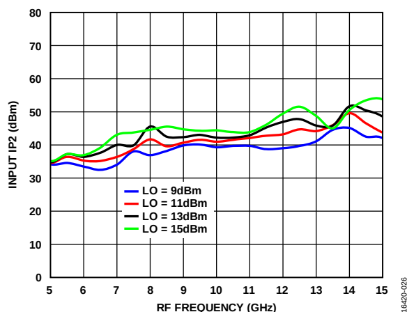
Figure 24. Input IP2 vs. RF Frequency at Various LO Power Levels, TA = 25°C
