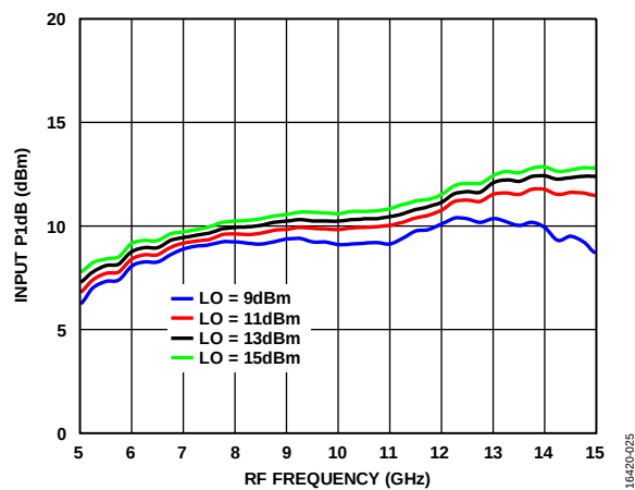
Figure 23. Input P1dB vs. RF Frequency at Various LO Power Levels, TA = 25°C
