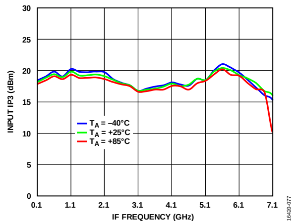
Figure 75. Input IP3 vs. IF Frequency at Various Temperatures, LO = 13 dBm
