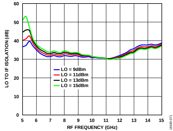
Figure 69. LO to IF Isolation vs. RF Frequency at Various LO Power Levels, T_A = 25^\circ\text{C}
