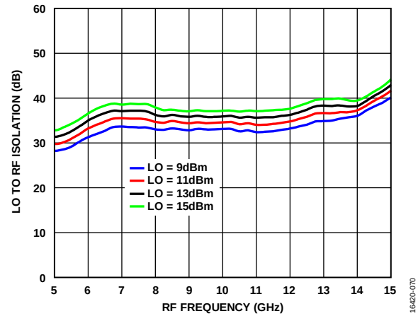
Figure 68. LO to RF Isolation vs. RF Frequency at Various LO Power Levels, T_A = 25^\circ\text{C}
