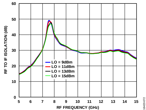
Figure 70. RF to IF Isolation vs. RF Frequency at Various LO Power Levels, T_A = 25^\circ\text{C}
