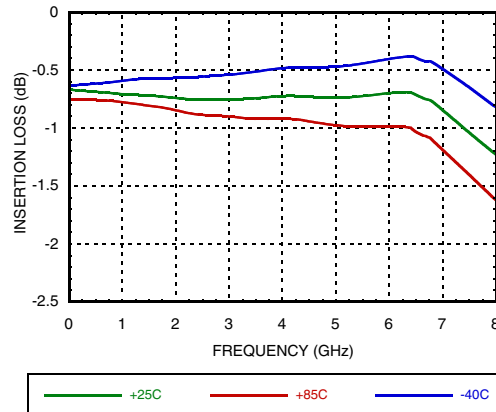
Insertion Loss
