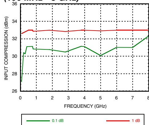
0.1 and 1 dB Input Compression Point, 5V (100 MHz - 8 GHz)
