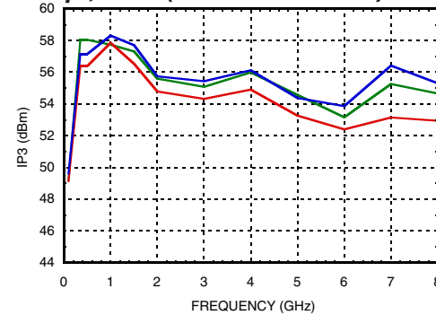
Input Third Order Intercept Point over Temp., 3.3V (100 MHz - 8 GHz)
