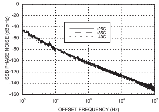
Typical SSB Phase Noise @ V_{\text{tune}} = +5\text{V}
