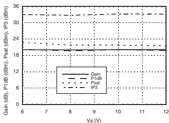
Gain, Power & Output IP3 vs. Supply Voltage for Constant Id= 74 mA @ 850 MHz
