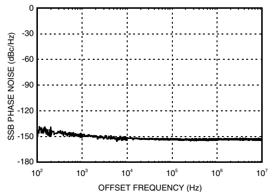
SSB Phase Noise Performance, \text{Pin} = 0\text{ dBm} , \text{Fin} = 6\text{ GHz} , T = 25^\circ\text{C}
