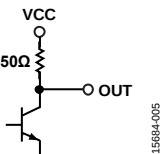
Figure 5. OUT Interface Schematic
