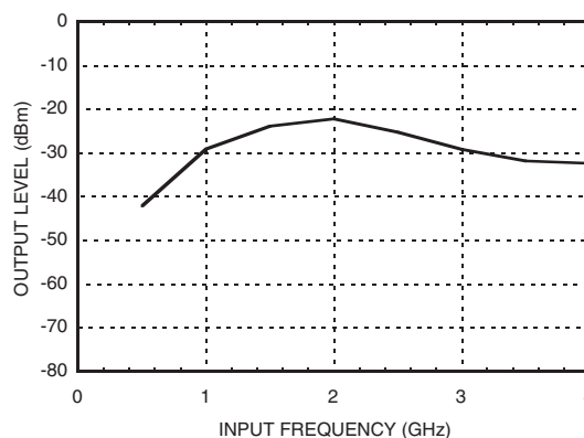
Reverse Leakage, P_{in} = 0\text{ dBm} , T = 25^\circ\text{C}
