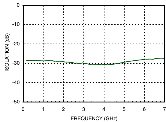
Reverse Isolation
