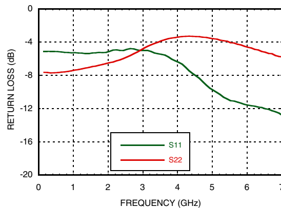
Input & Output Return Loss
