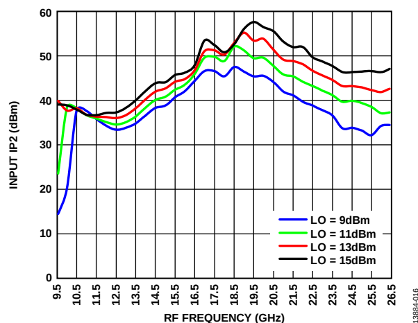
Figure 16. Input IP2 vs. RF Frequency at Various LO Power Levels, TA = 25°C
