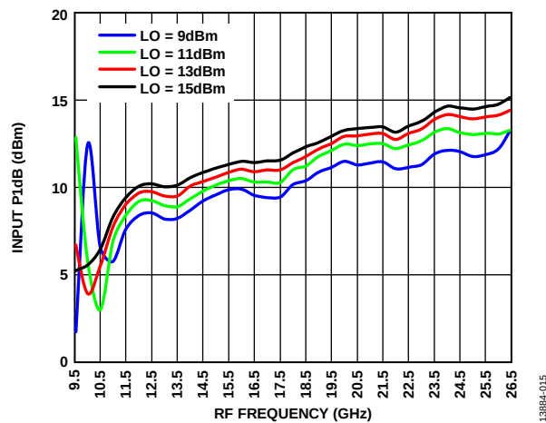
Figure 15. Input P1dB vs. RF Frequency at Various LO Power Levels, TA = 25°C
