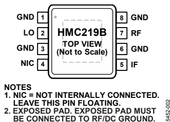
Figure 2. Pin Configuration
