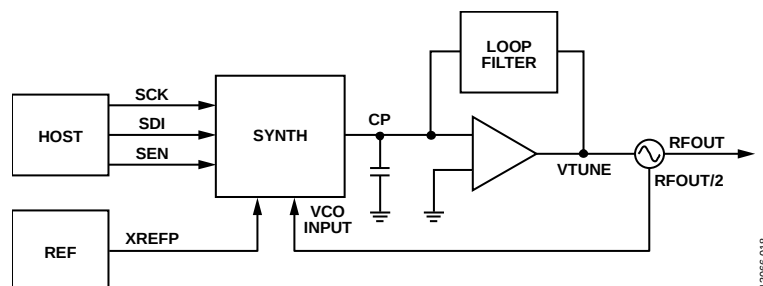
Figure 16. Typical Application Diagram
