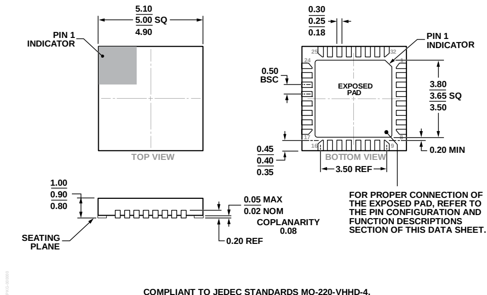
Figure 18. 32-Lead Lead Frame Chip Scale Package [LFCSP_VQ] 5 mm × 5 mm Body, Very Thin Quad (HCP-32-1) Dimensions shown in millimeters
