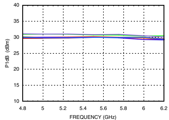
Input P1dB, Major States Only
