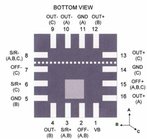
HMC1053 Pinout
