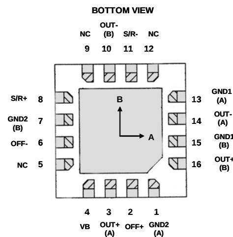
HMC1053 Pinout
