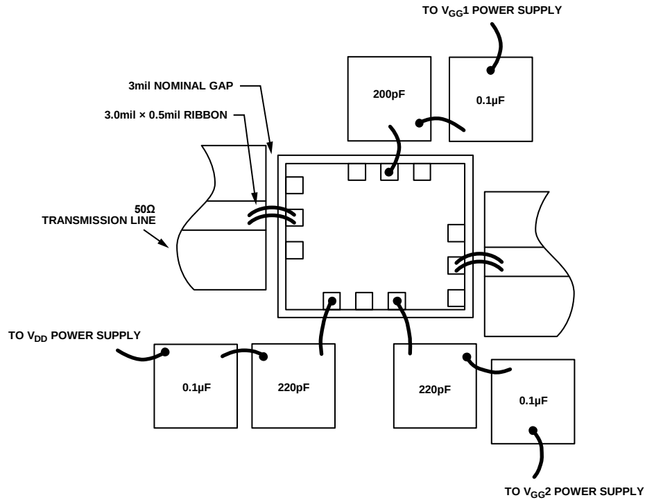
Figure 24. Assembly Diagram
