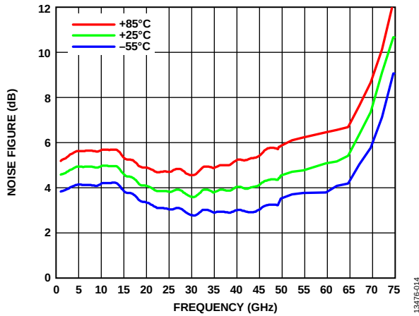
Figure 14. Noise Figure
