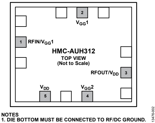
Figure 2. Pin Configuration
