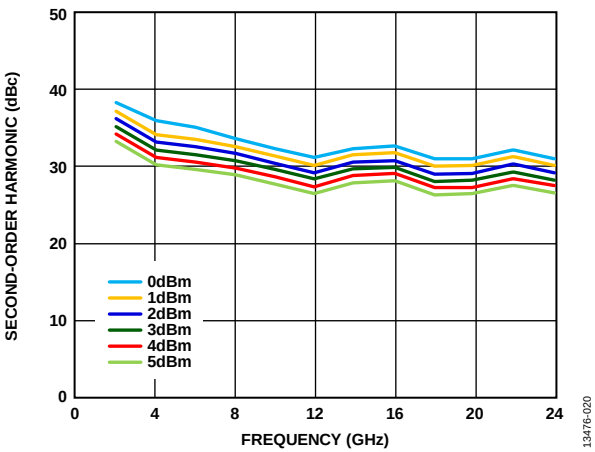
Figure 20. Second-Order Harmonic vs. Frequency at Various P_{OUT} Levels
