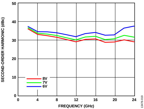
Figure 19. Second-Order Harmonic vs. Frequency at Various Supplies ( V_{DD} ), P_{OUT} = 2\text{ dBm}
