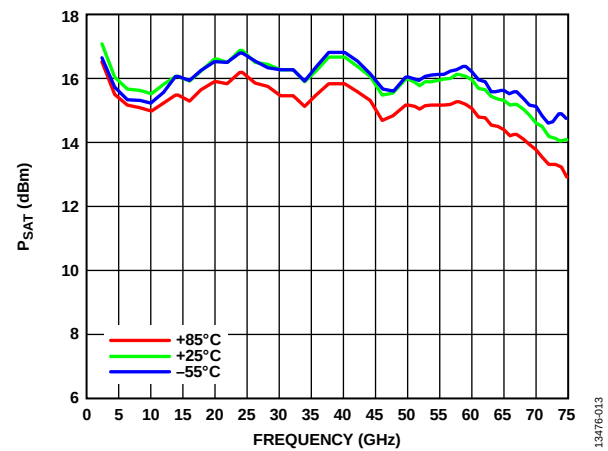
Figure 13. P_{SAT} vs. Frequency at Various Temperatures
