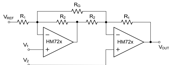
Figure 6. Instrumentation Amplifier
