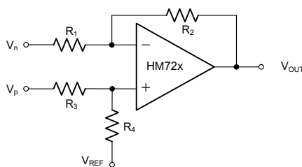
Figure 5. Differential Amplifier
