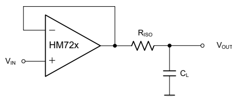
Figure 3. Indirectly Driving Heavy Capacitive Load
