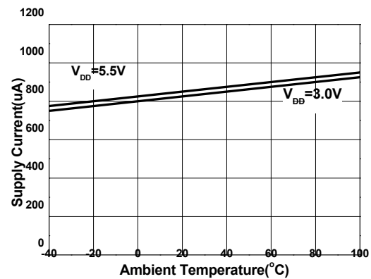
Quiescent Current as a function of Temperature.
