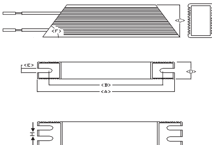
B Type Narrow base
