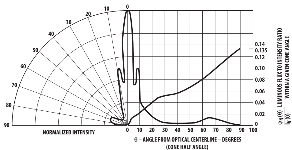
Figure 7. Relative luminous intensity vs. angular displacement.
