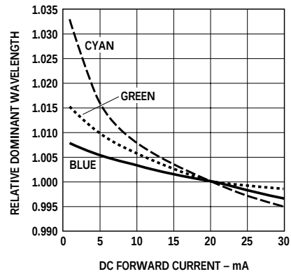
Figure 4. Relative dominant wavelength vs. DC forward current.
