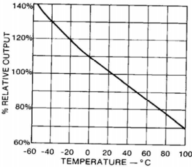
Fig. 7. Output vs. Temperature C654B
