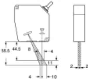
HL-C105B-BK, HL-C105F-BK HL-C105B, HL-C105F
