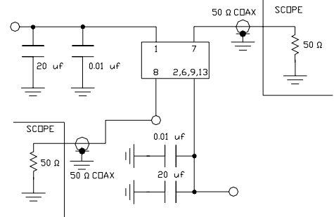
TEST CIRCUIT
