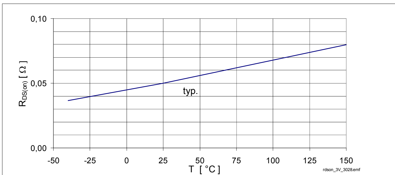
Figure 10 Typical On-State Resistance, R_{DS(on)} = f(T_J) , V_{IN} = 3V
