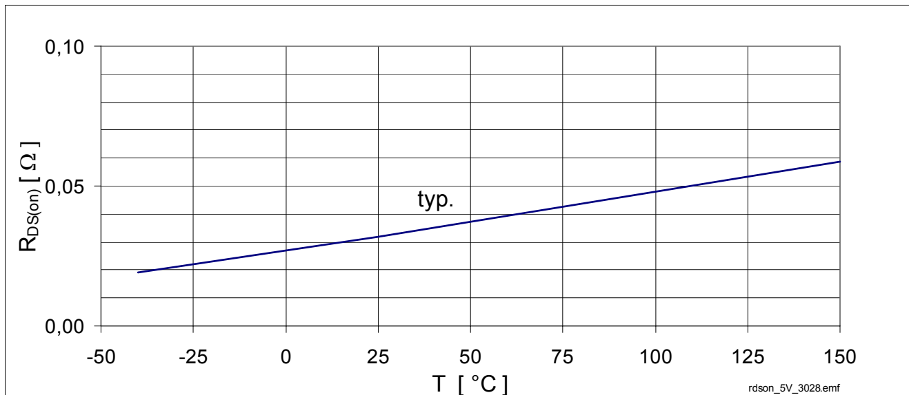
Figure 9 Typical On-State Resistance, R_{DS(on)} = f(T_J) , V_{IN} = 5V
