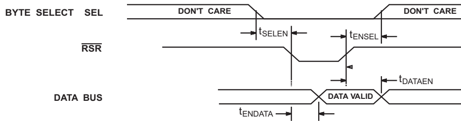
STATUS REGISTER READ CYCLE
