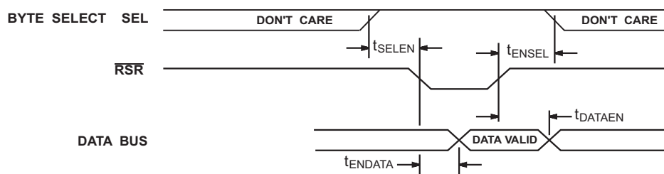
CONTROL REGISTER READ CYCLE
