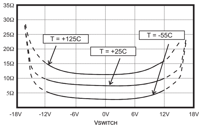
Typical R_{ON} as a function of V_{SWITCH} and Temperature (10mA switch current, V_{SUPPLY} = +3.3\text{V} )
