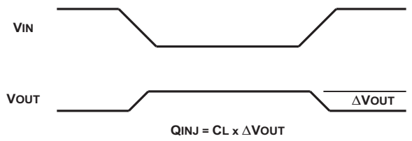
Figure 5. Charge Injection
