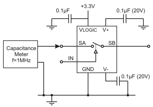
Figure 8 - Off Capacitance
