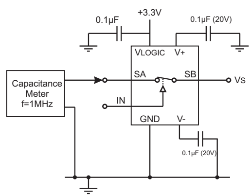
Figure 9 - On Capacitance
