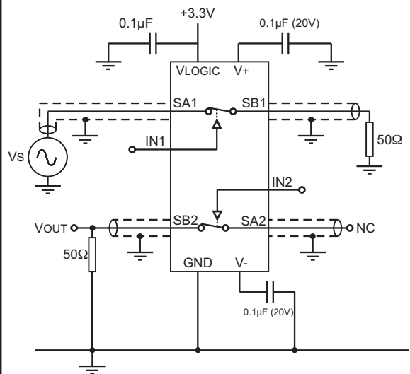
Figure 7 - Channel-to-Channel Crosstalk
