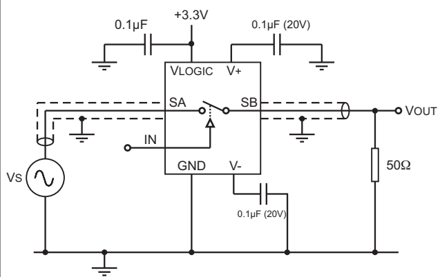
Figure 6 - Off Isolation
