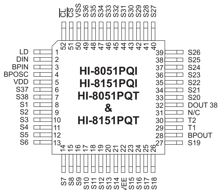
52 Pin Plastic PQFP
