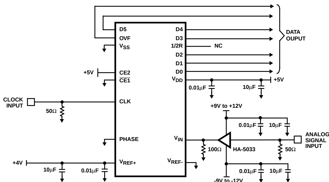
FIGURE 13. TEST CIRCUIT
