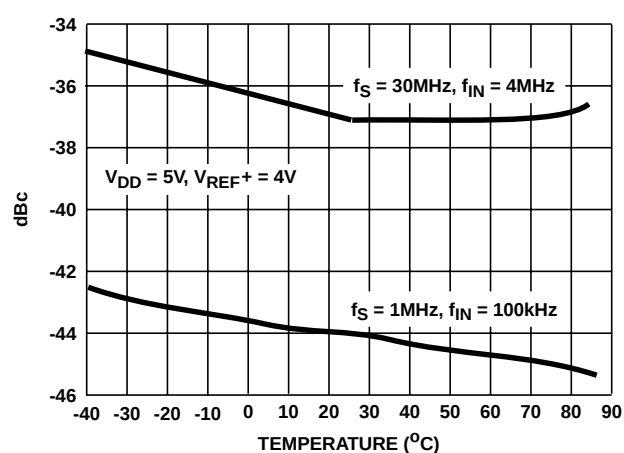
FIGURE 6. TOTAL HARMONIC DISTORTION vs TEMPERATURE
