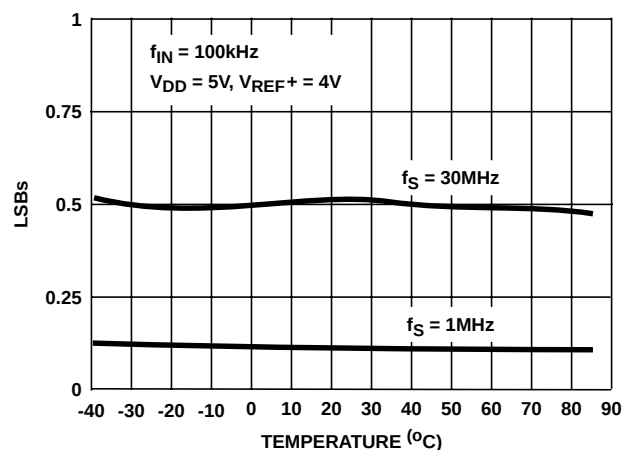
FIGURE 8. DNL vs TEMPERATURE
