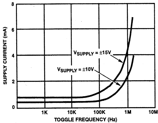
FIGURE 5A. SUPPLY CURRENT vs TOGGLE FREQUENCY
