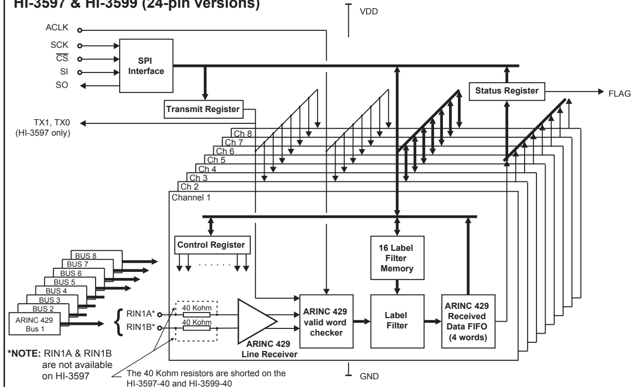
Figure 1. Block Diagrams
