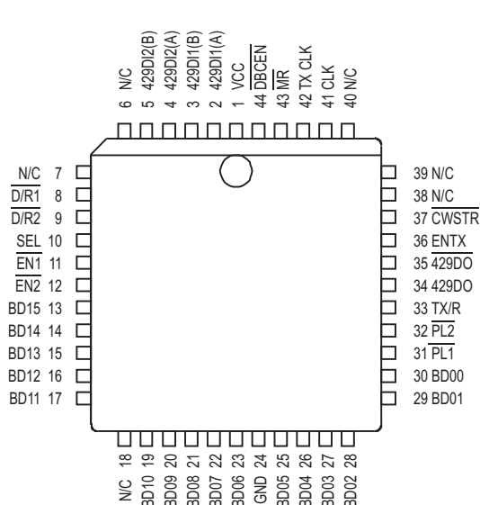
HI-3282PJI / HI-3282BPJI HI-3282PJT / HI-3282BPJT HI-3282PJI-10 / HI-3282BPJI-10 HI-3282PJT-10 / HI-3282BPJT-10 44-Pin J-Lead PLCC
