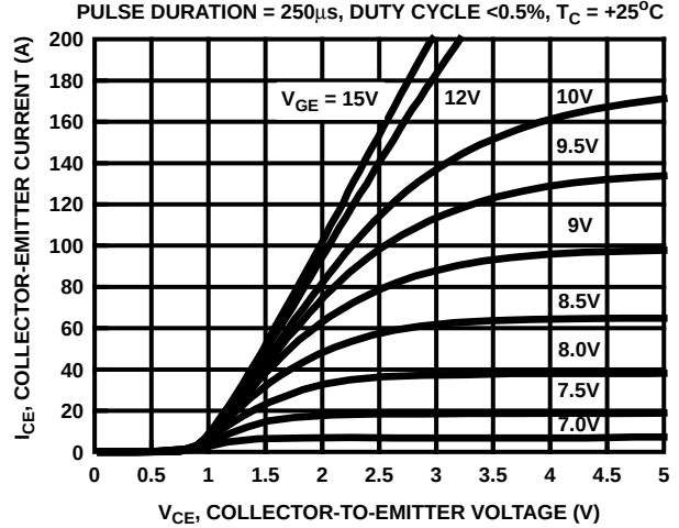
FIGURE 2. SATURATION CHARACTERISTICS
