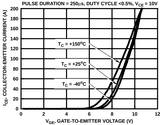
FIGURE 1. TRANSFER CHARACTERISTICS
