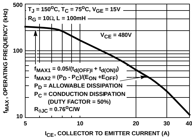
FIGURE 13. OPERATING FREQUENCY vs COLLECTOR TO EMITTER CURRENT T
