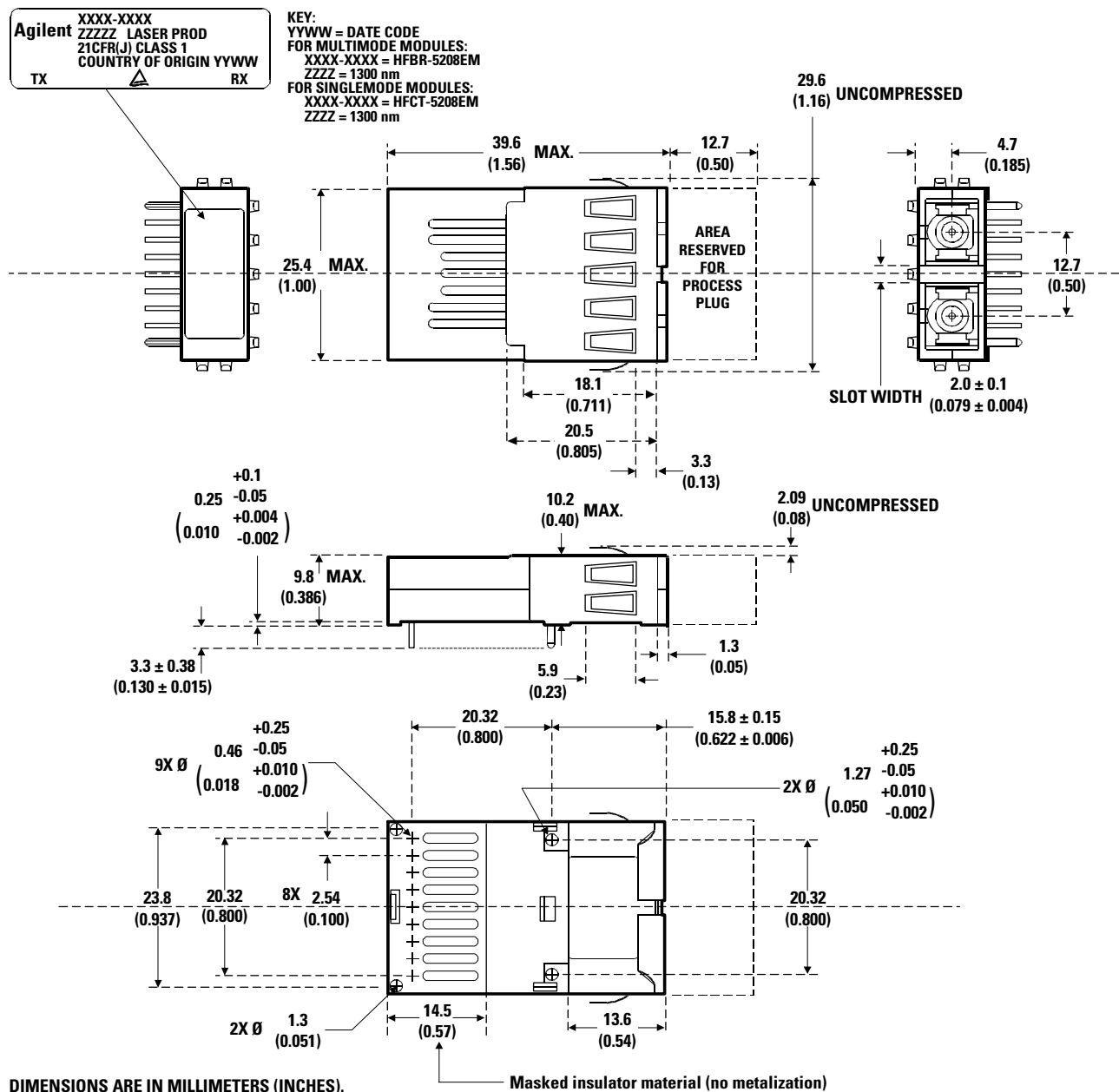
Figure 8. Package Outline for HFBR/HFCT-5208EM
