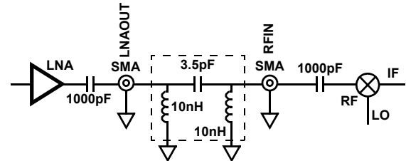
FIGURE 36. HFA3600 HIGH PASS FILTER IMPLEMENTATION
