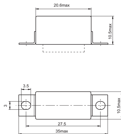
Mounting style 1
