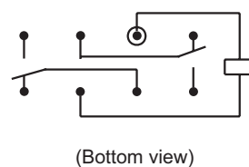
Wiring Diagram
