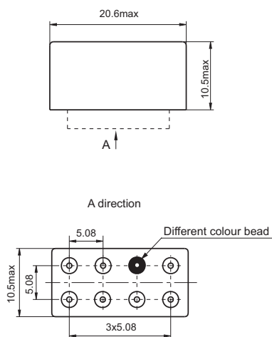
Mounting style 0
