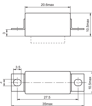
Mounting style 2
