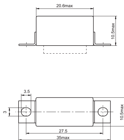
Mounting style 1
