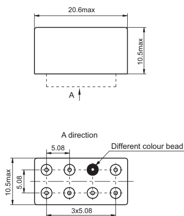
Mounting style 0
