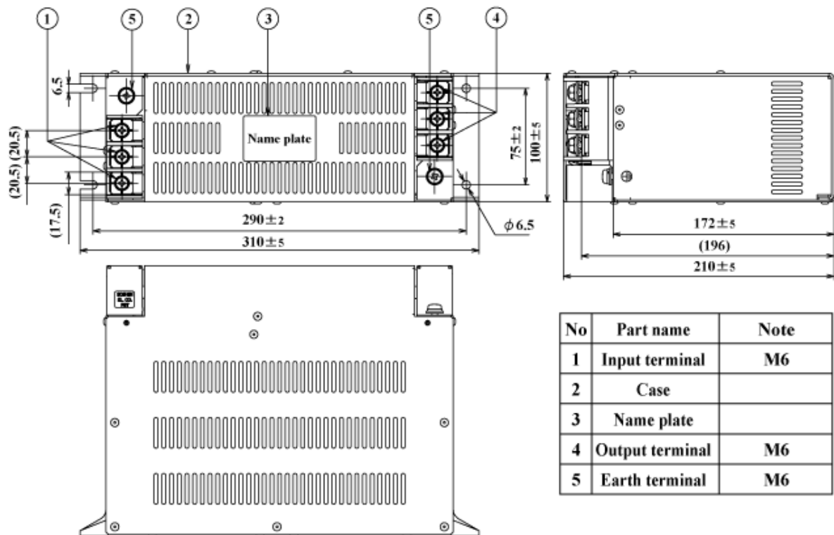
fig.3 (80A, 100A)
