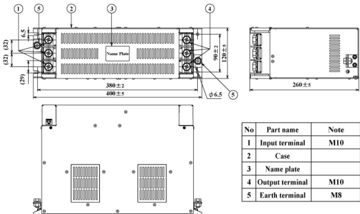
fig.5 (200-300A)
