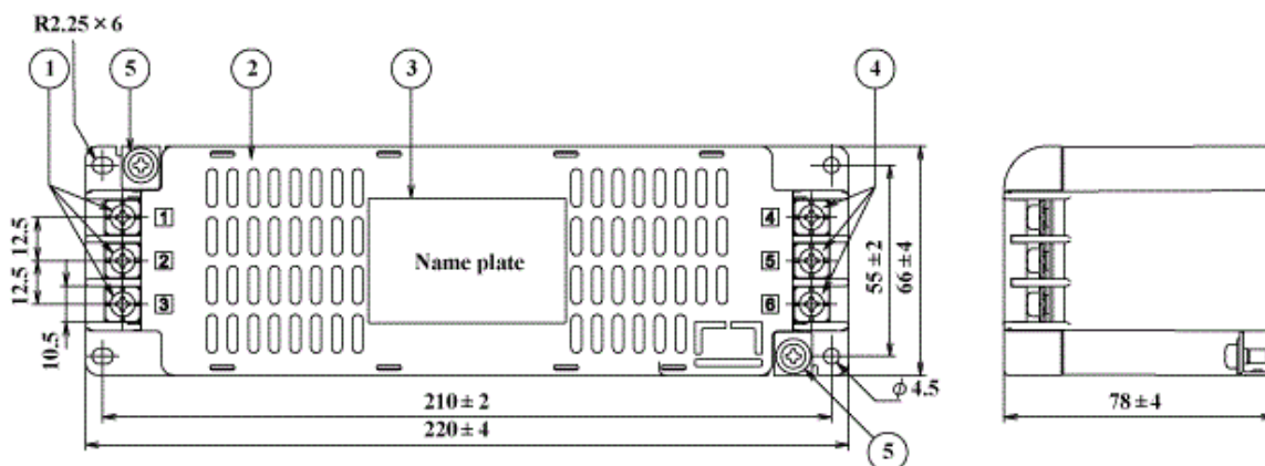
fig.1 (10-30A)
