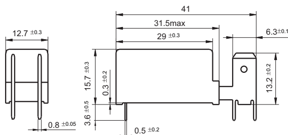
Quick connect terminals vertical
