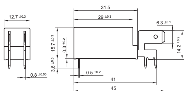
Quick connect terminals horizontal
