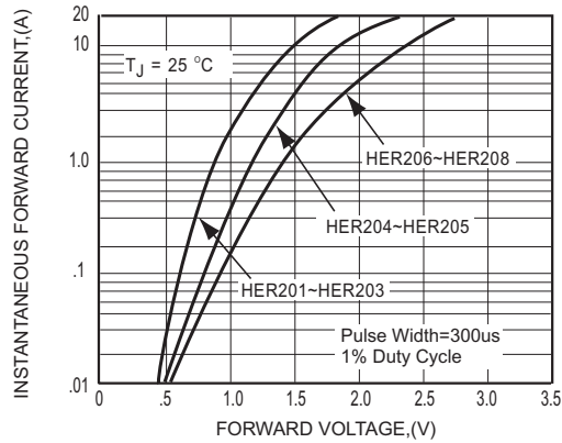
FIG.1-TYPICAL FORWARD CHARACTERISTICS
