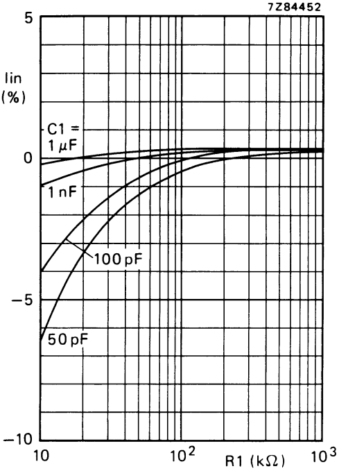
Fig.15 VCO frequency linearity as a function of R1; R2 = ∞; VDD = 10 V.
