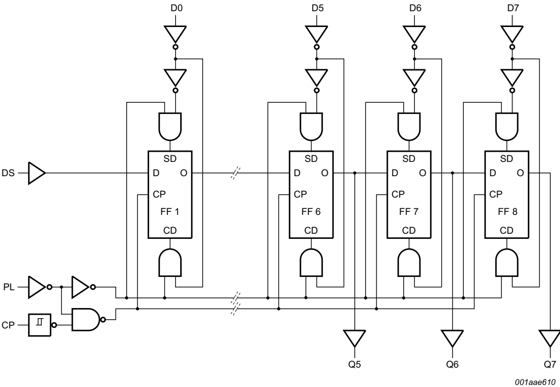
Fig 2. Logic diagram
