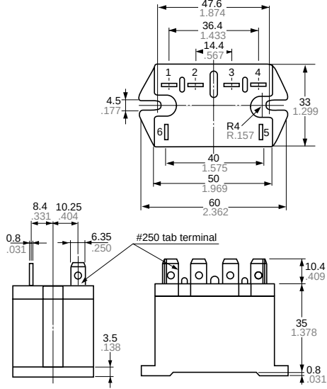
2 Form A
