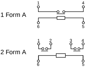
Schematic (Bottom view) Single side stable type
