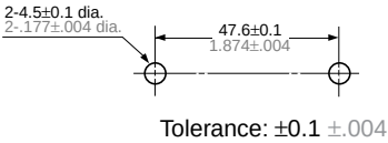
Panel cutout
