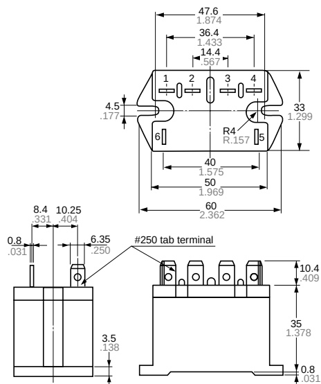
2 Form A
