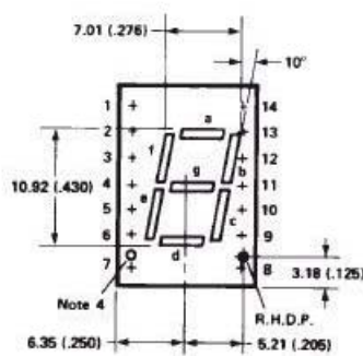
J, K FRONT VIEW
