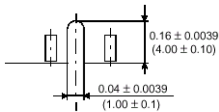
Detail Z
