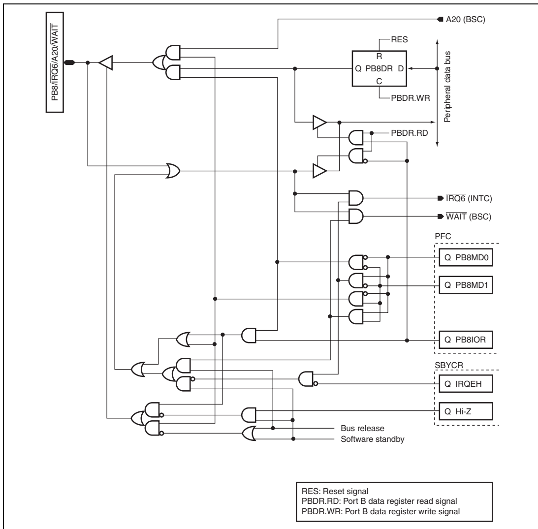
Figure D.20 PB8/ \overline{\text{TRQ6}} /A20/ \overline{\text{WAIT}}
