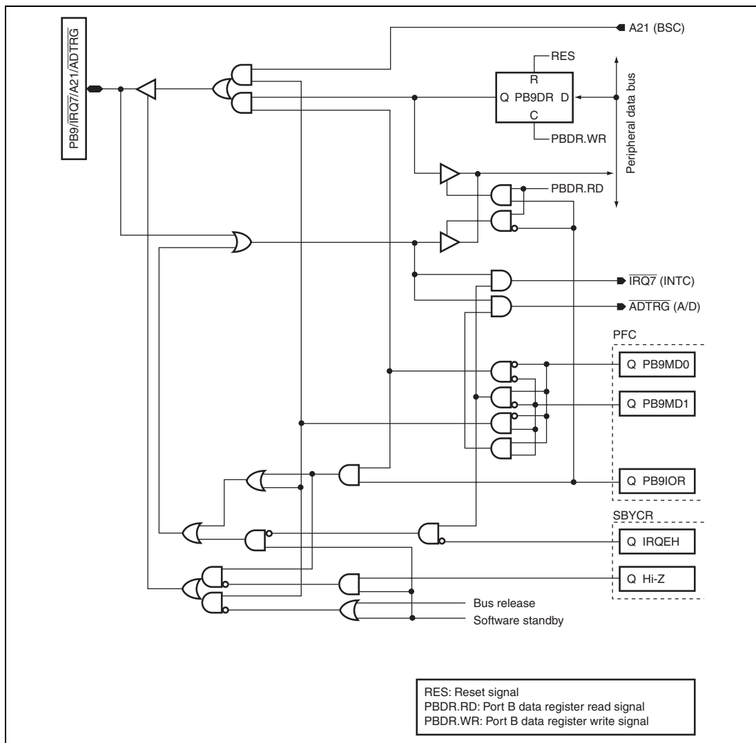
Figure D.21 PB9/ \overline{\text{TRQ7}} / \overline{\text{A21}} / \overline{\text{ADTRG}}
