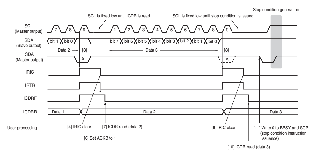
Figure 14.12 An Example of the Stop Condition Issuance Timing in Master Receive Mode (MLC = WAIT = 0, HNDS = 1)
