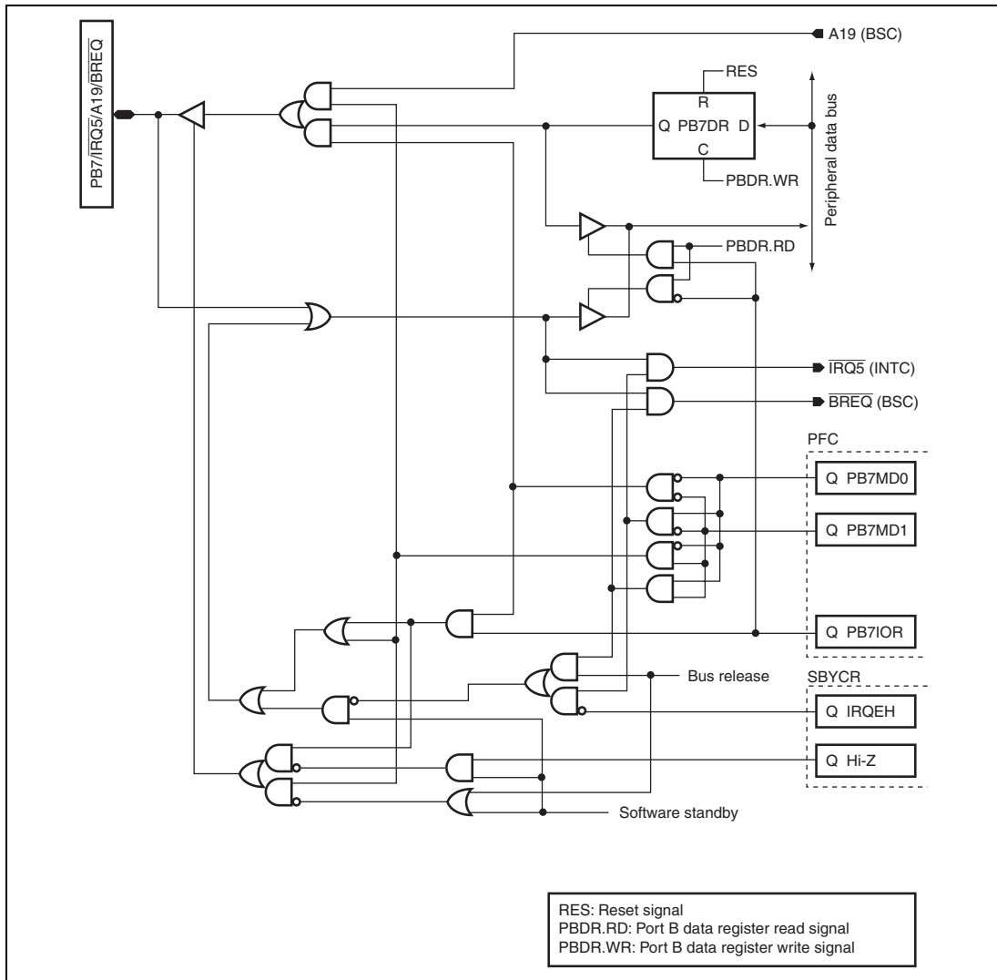
Figure D.19 PB7/ \overline{\text{TRQ5}} / \text{A19} / \overline{\text{BREQ}}
