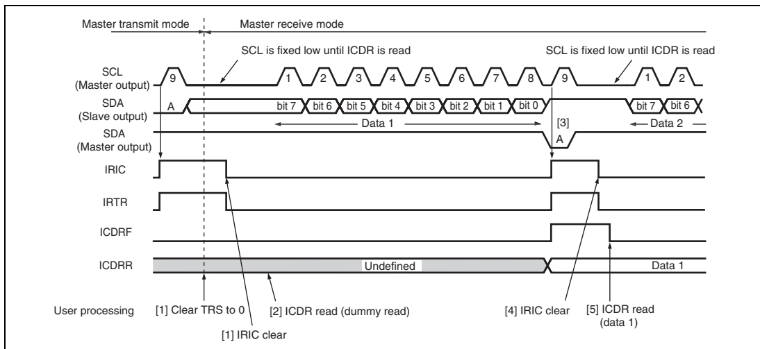
Figure 14.11 An Example of the Timing of Operations in Master Receive Mode (MLC = WAIT = 0, HNDS = 1)
