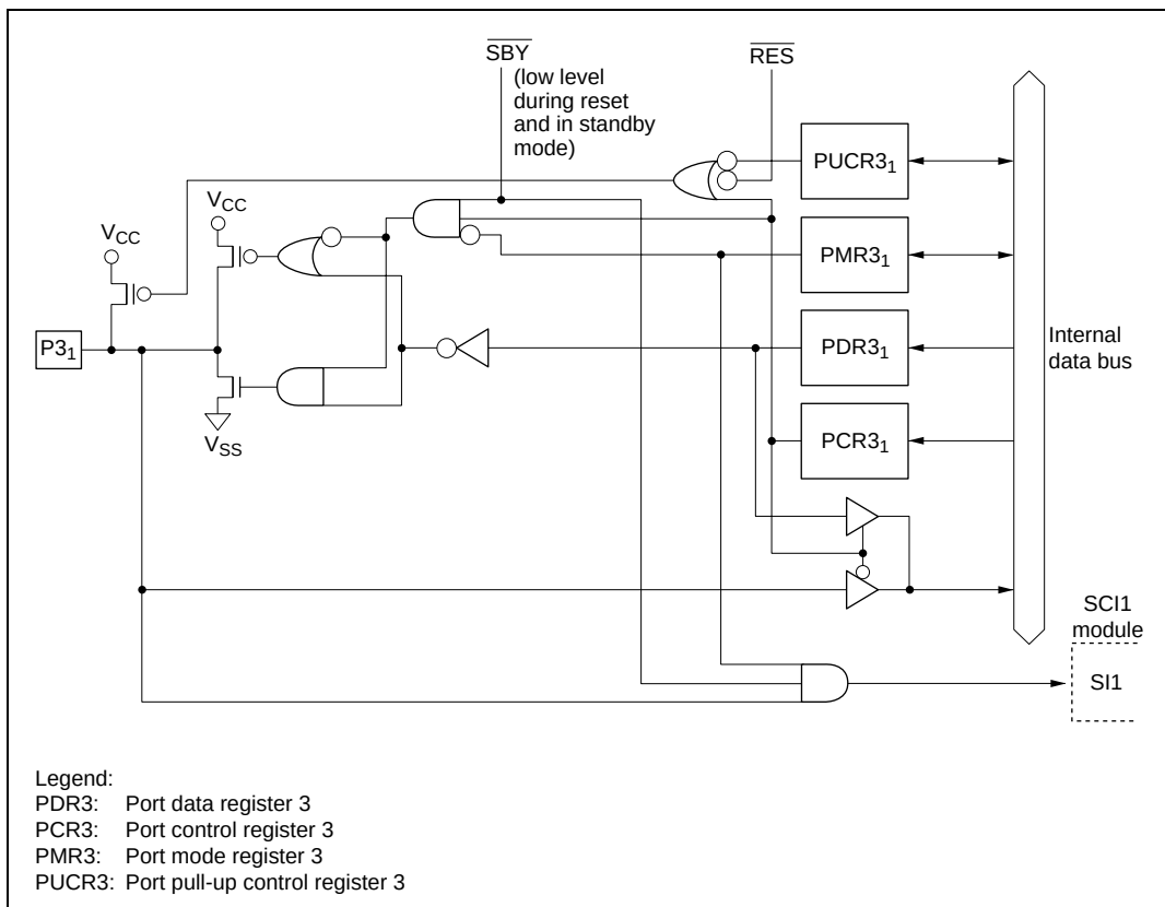
Figure C.3 (b) Port 3 Block Diagram (Pin P3 1 )
