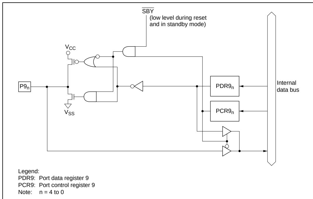
Figure C.8 Port 9 Block Diagram (Pins P9_4 to P9_0 )
