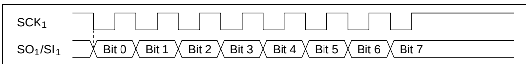
Figure 10.2 Transfer Format
