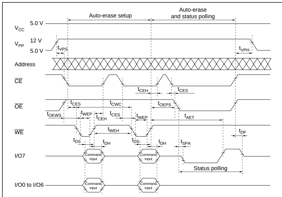
Figure 6.20 Auto-Erase Timing
