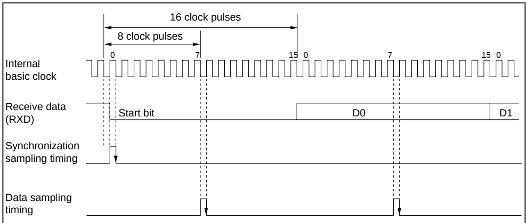
Figure 10.26 Receive Data Sampling Timing in Asynchronous Mode
