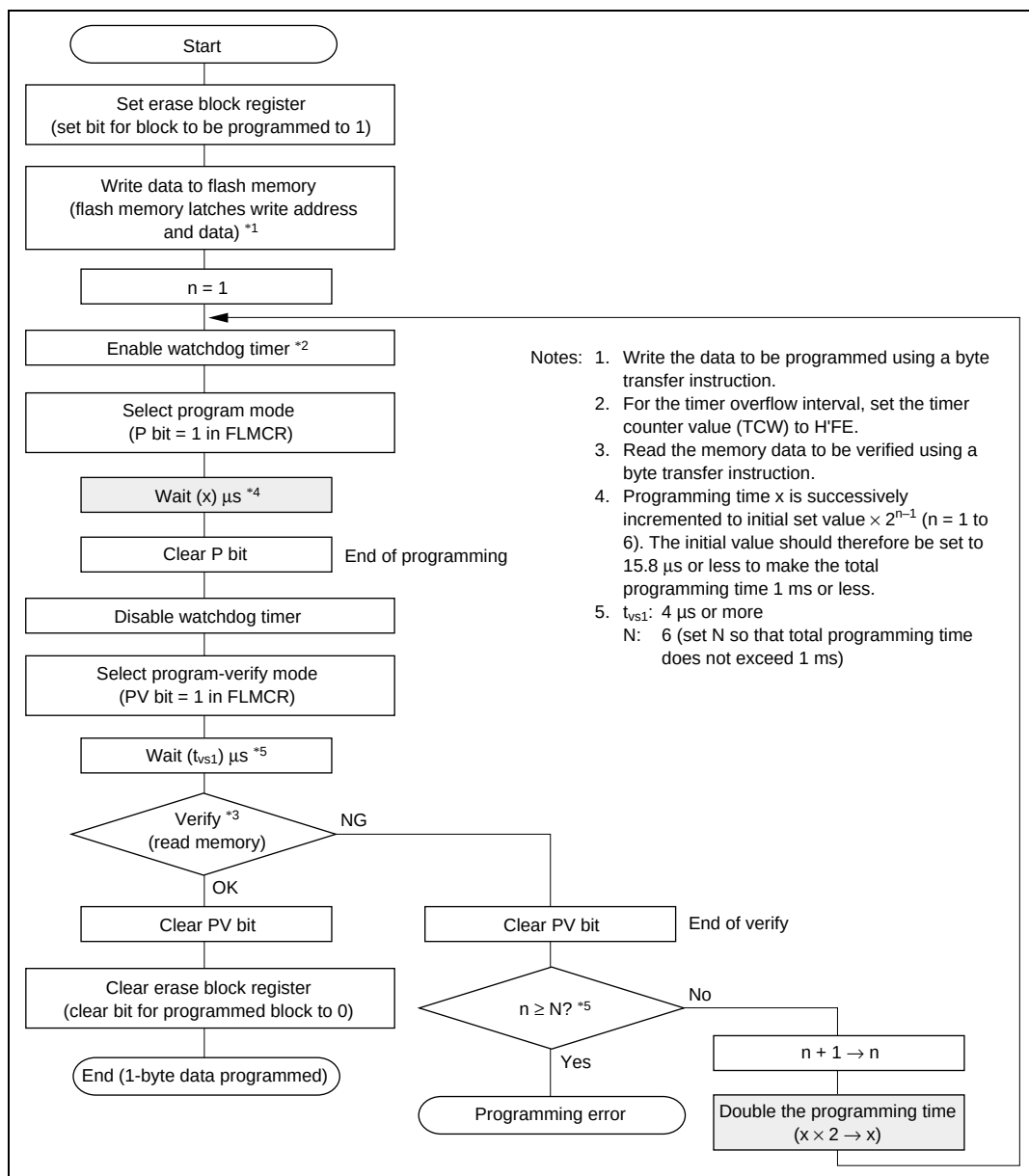
Figure 6.13 Programming Flowchart
