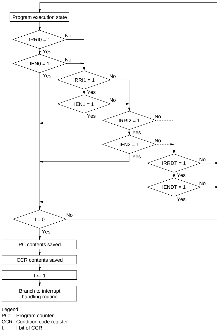
Figure 3.3 Flow up to Interrupt Acceptance
