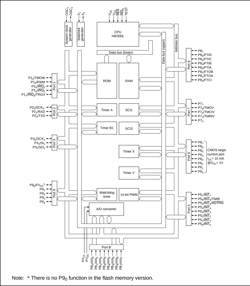
Figure 1.1 Block Diagram
