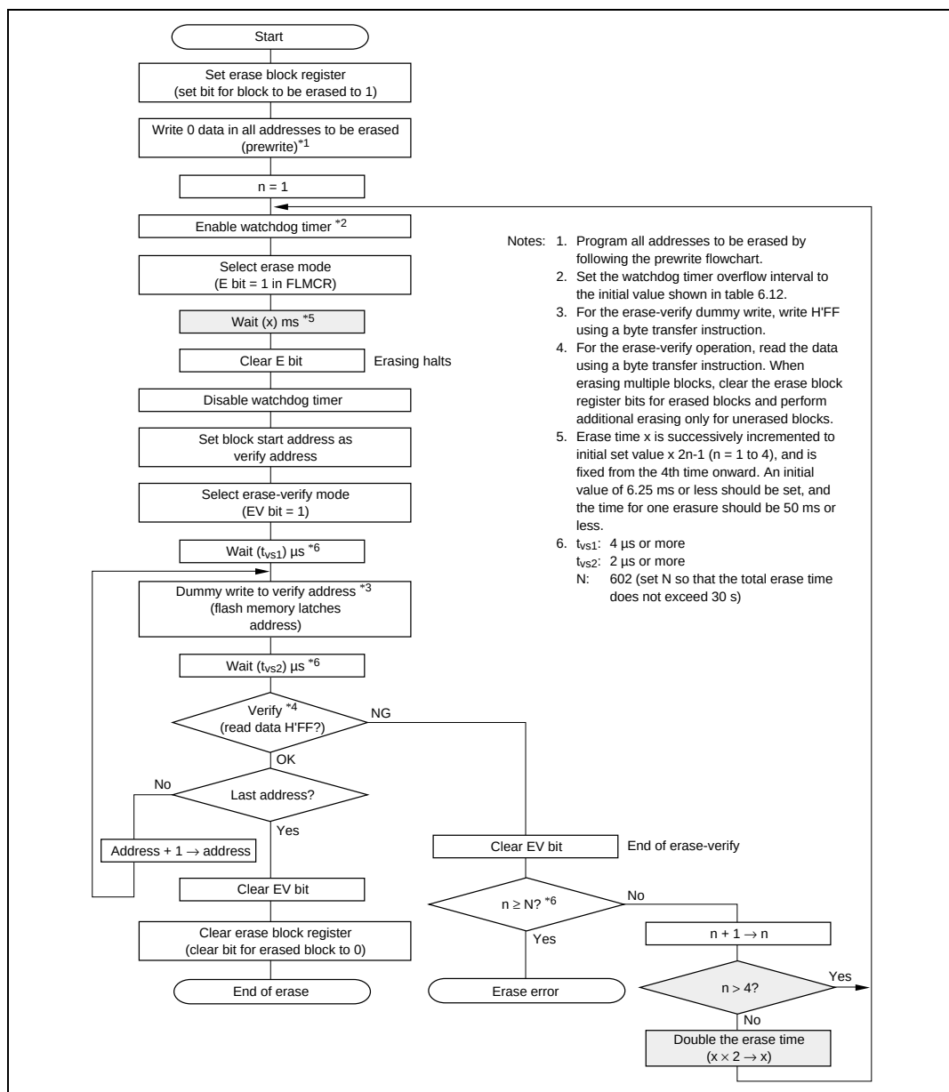
Figure 6.14 Erase Flowchart
