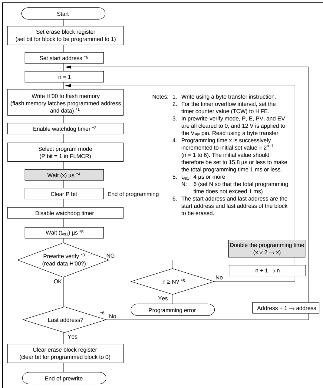
Figure 6.15 Prewrite Flowchart
