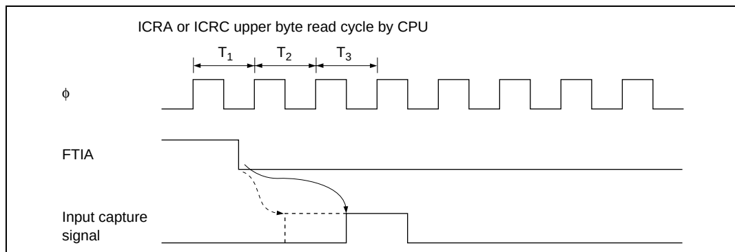
Figure 9.27 Buffered Input Capture Signal Timing (during ICRA or ICRD Read)
