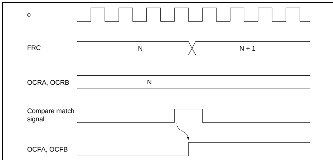
Figure 9.29 OCFA and OCFB Set Timing
