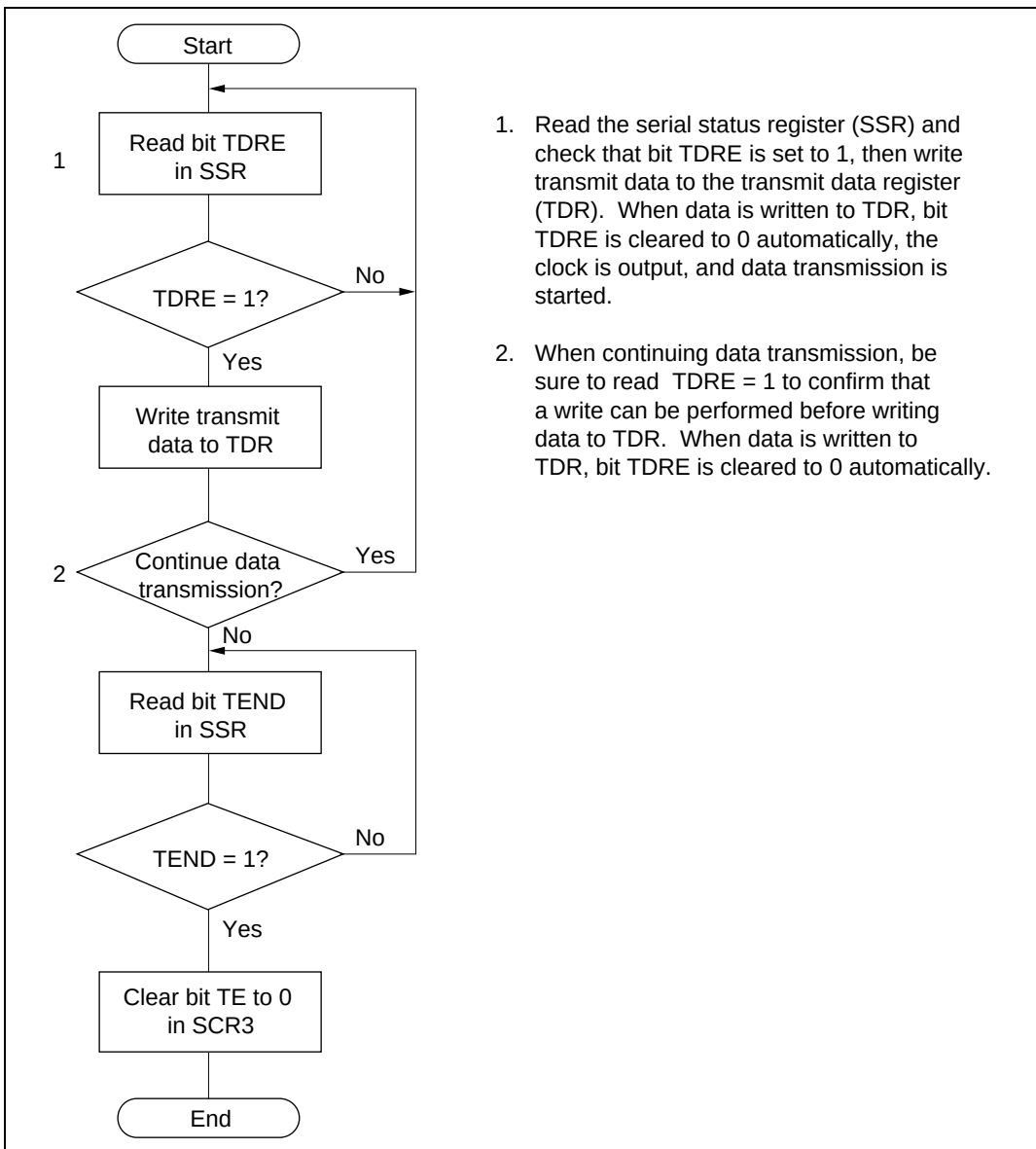
Figure 10.16 Example of Data Transmission Flowchart (Synchronous Mode)
