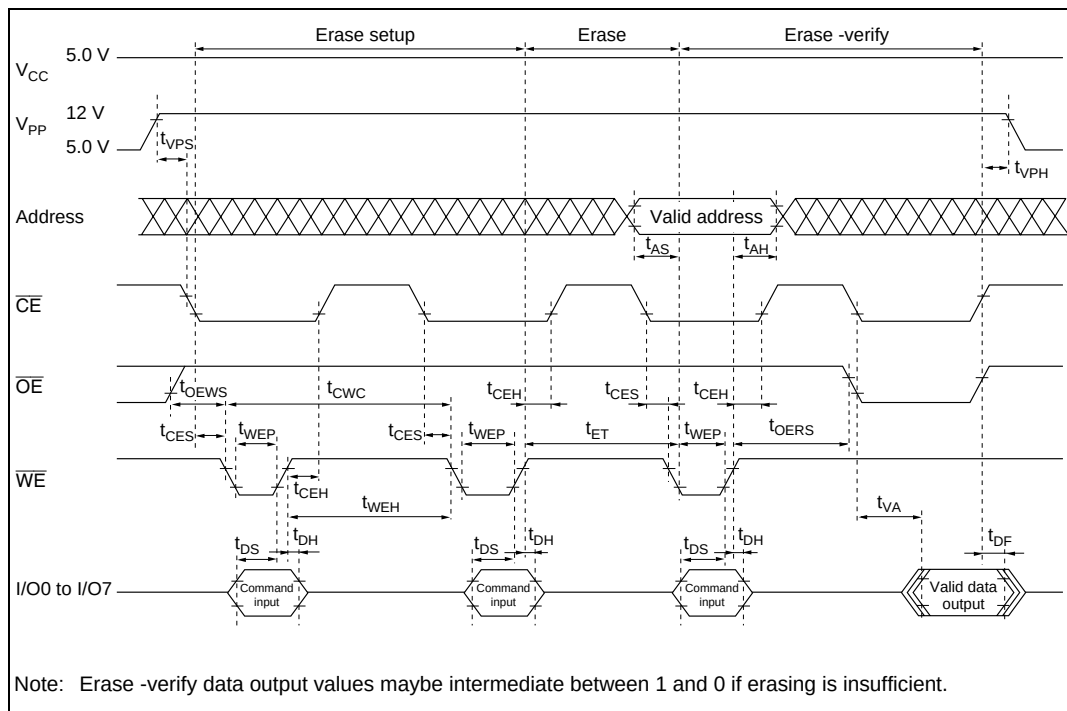
Figure 6.22 Erase Timing
