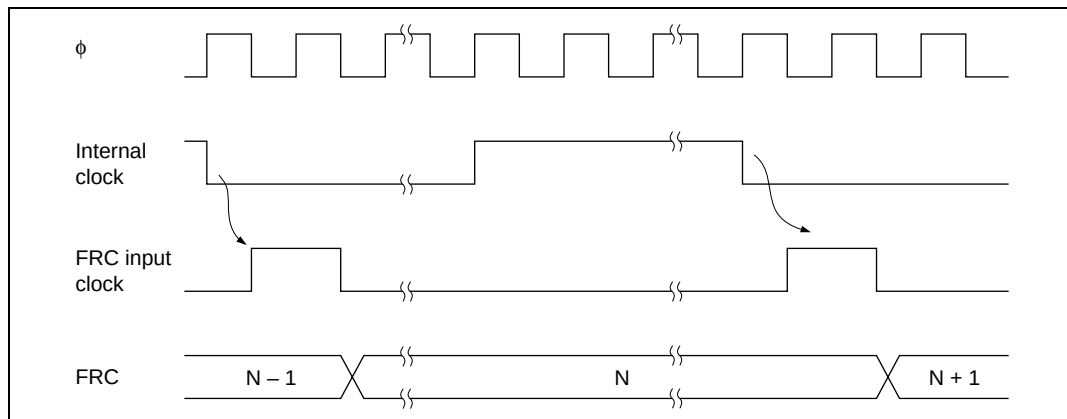
Figure 9.20 Increment Timing with Internal Clock
