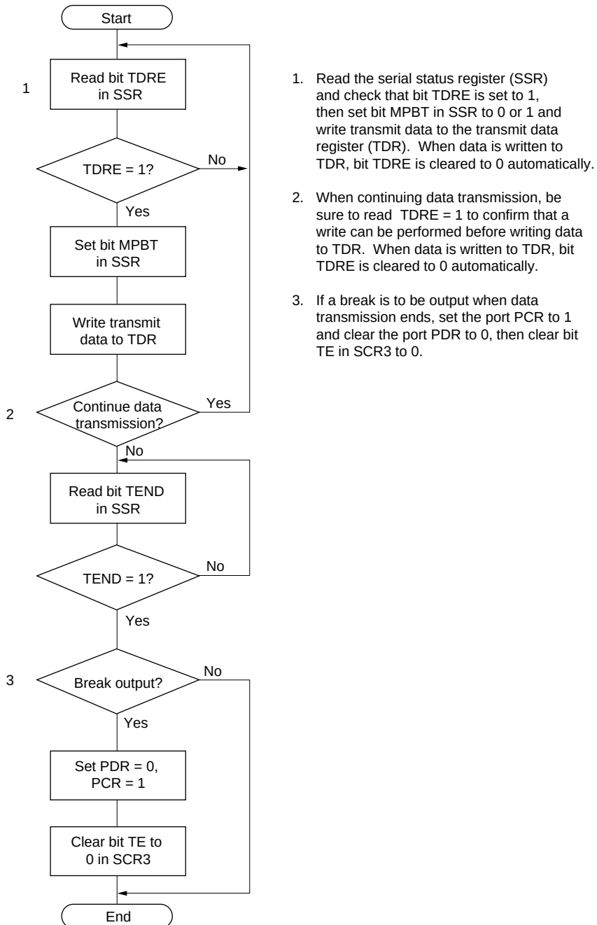
Figure 10.22 Example of Multiprocessor Data Transmission Flowchart
