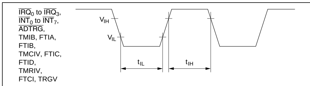
Figure 13.3 Input Timing
