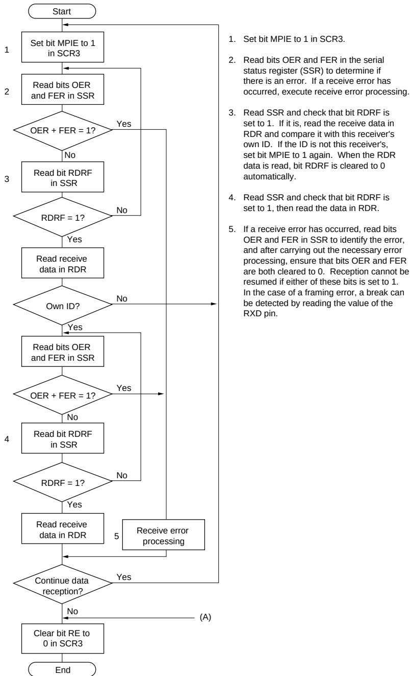
Figure 10.24 Example of Multiprocessor Data Reception Flowchart
