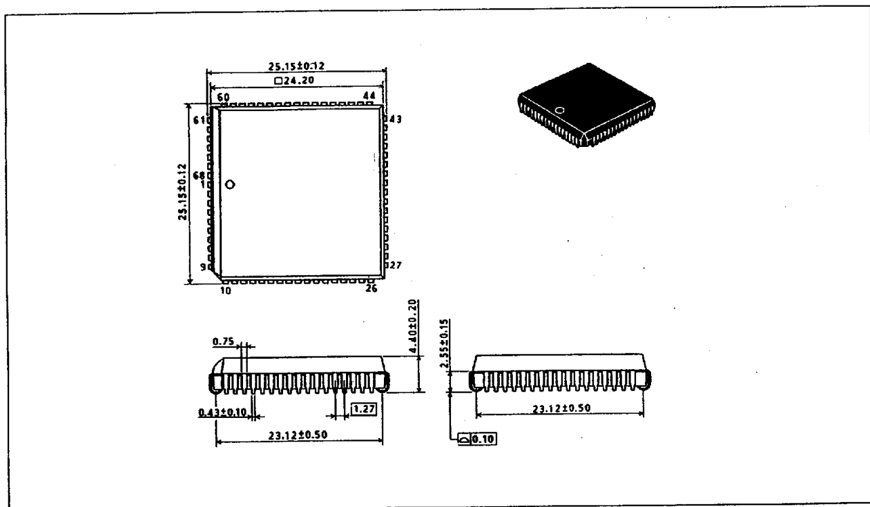
Figure F-4 Package Dimensions (CP-68)
