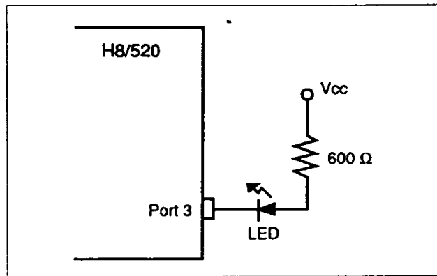
Figure 18-2 Example of Circuit for Driving an LED
