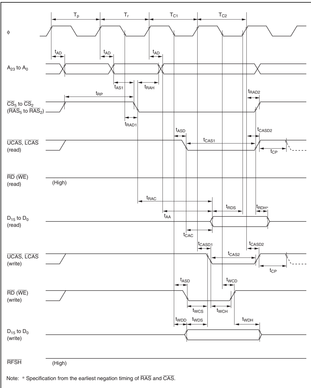
Figure 20.14 DRAM Bus Timing (Read/Write)
